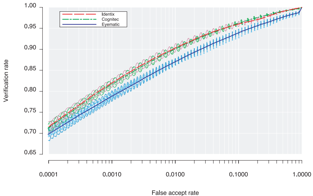
Fig. 8. Standard error ellipses for verification performance for Cognitech, Eyematic, and Identix. The standard error was computed from twelve HCInt small galleries of size 3,000. The center line is the ROC performance for the aggregate of all twelve galleries. The ellipses are two times the standard deviation at selected performance points, and the points clustered around the ellipses represent the performance of one of the twelve galleries at the selected performance point.
